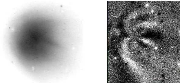
Figure 3: Comet Halley in 1910. Left: from a Vatican Astrograph plate. Right: from a Catania Astrograph plate, after a Sekanina-type filtering (courtesy G. Cremonese and R. Ligustri)
