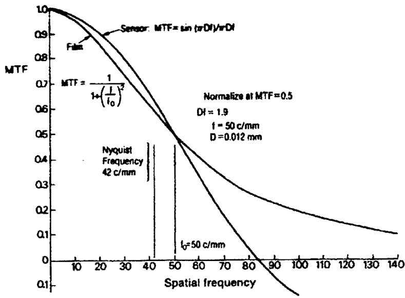
Figure 4: A method to calculate the effective pixel size that can be associated with photographic film when a frame transfer device with square pixels is assumed as the sensor model. The curve shown for film is based on a theoretical model and does not represent a particular film
