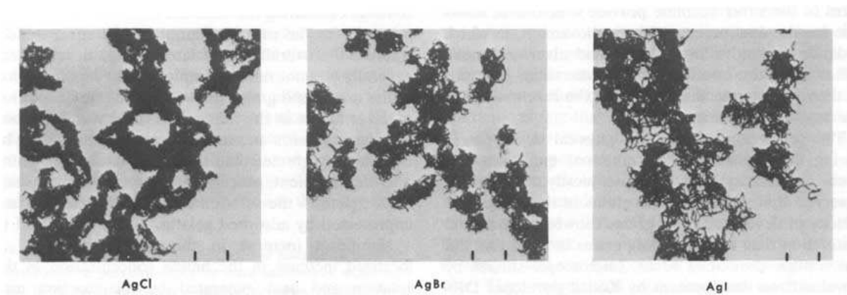
Figure 3: Different halides have somewhat different filament growth patterns. Left to right: AgCl, AgBr, AgI
